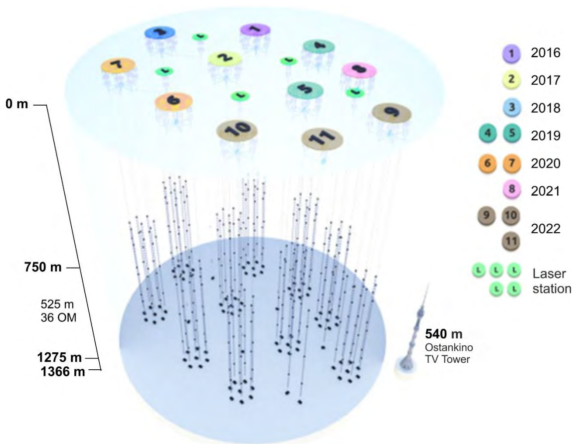
Fig. 10. Telescope deployment status as of late 2022. The setup contains 2916 optical modules and seven laser calibration light sources at five stations
