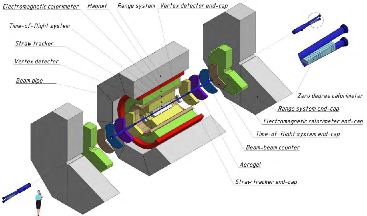
Fig. 5. General scheme of the Spin Physics Detector (SPD)
