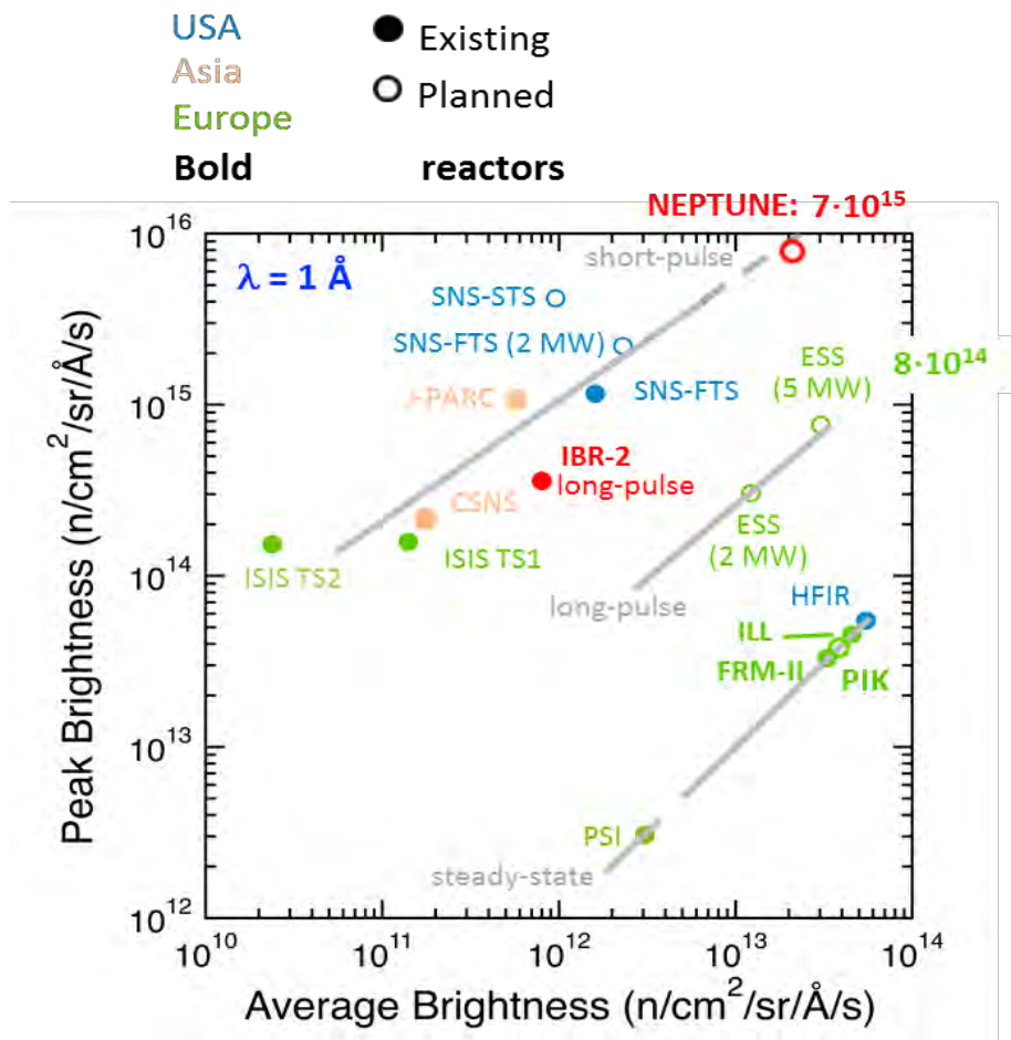
Fig. 9. Pulsed and average brightness for thermal neutrons of the IBR-2 reactor and the developed NEPTUNE source in comparison with neutron sources of various neutron centers
