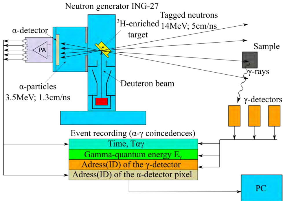
Fig. 23. Scheme of experiments using the tagged neutron method to study the interaction of fast neutrons with nuclei
