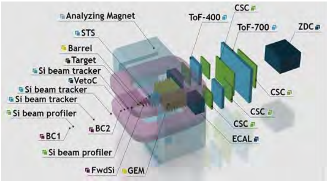
Fig. 3. Full configuration of BM@N detectors for implementation of research with heavy ion beams
