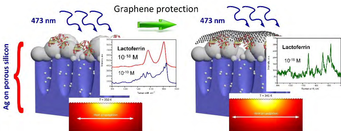
Fig. 30. Biosensing: ultrasensitive detection of organic molecules
