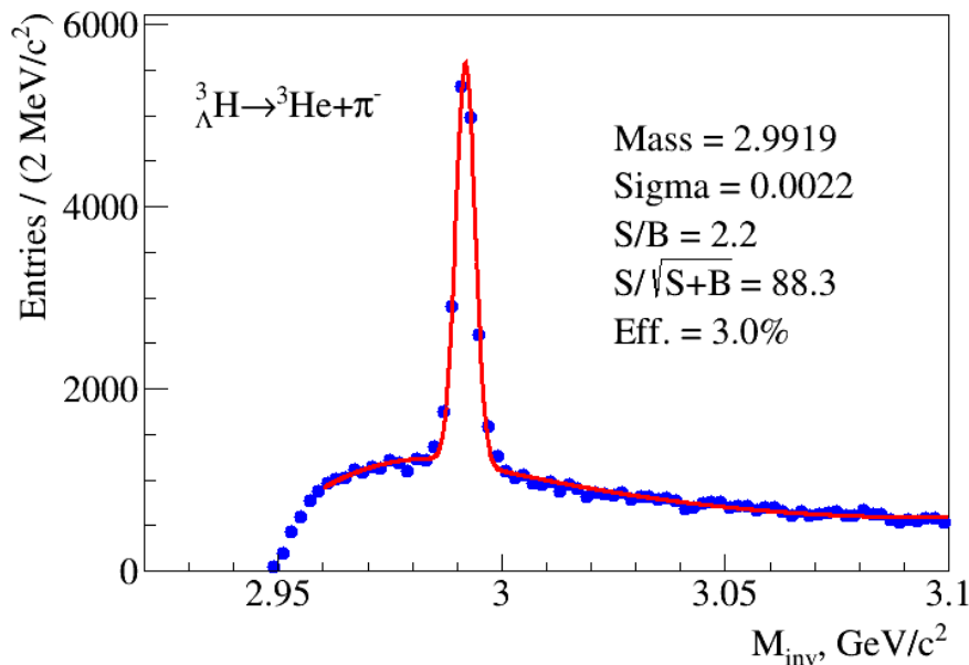
Fig. 13. To evaluate the prospects for studying hypernuclei at NICA, a detailed simulation of the MPD detector parameters was performed for the reconstruction of hypertritons in Bi+Bi collisions at a centre-of-mass energy of 9.2 \cdot A GeV. The distribution of the reconstructed invariant mass of the hypertriton in two-body decay mode is shown for the statistics of 40 million Bi+Bi collisions
