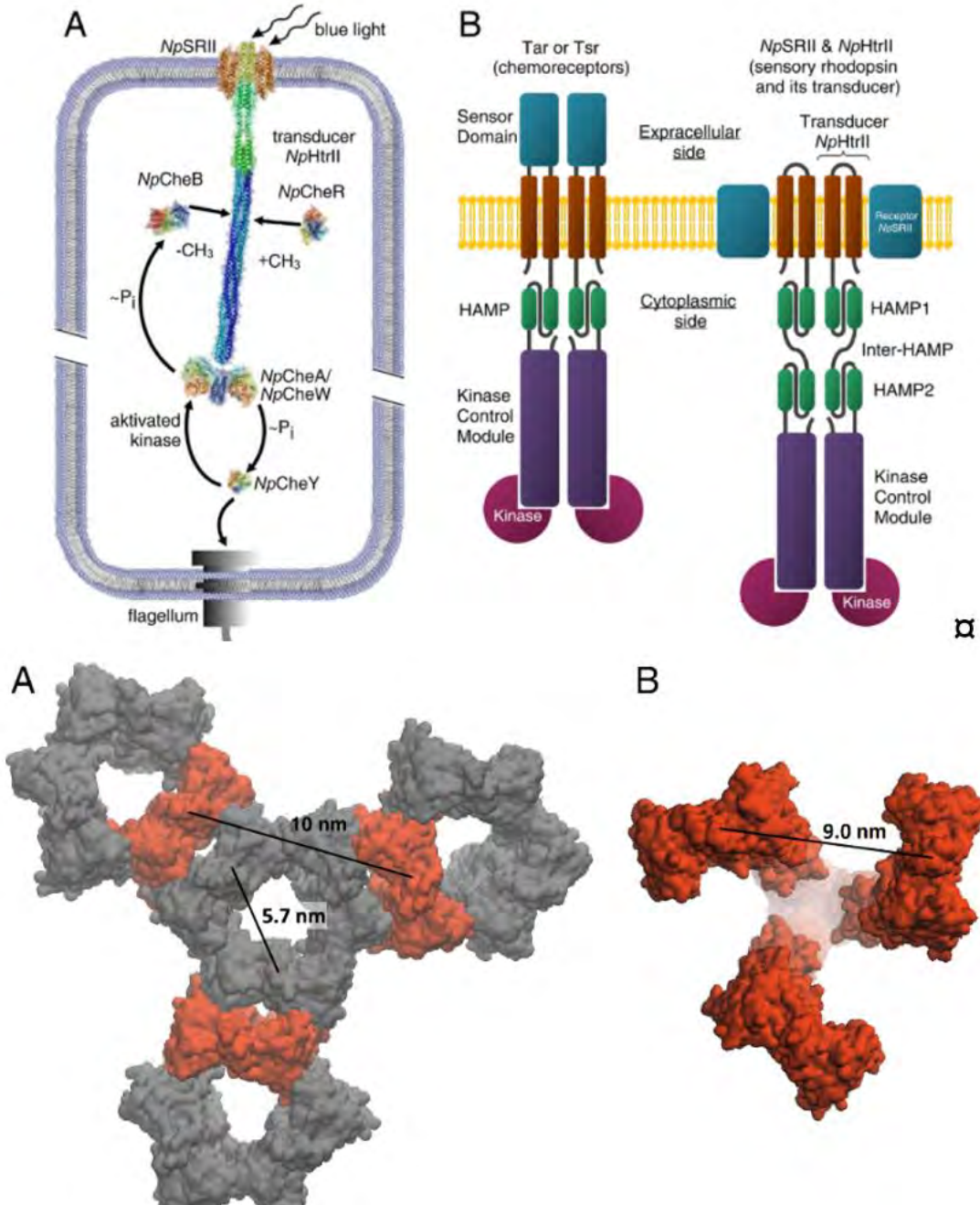
Fig. 28. Study of the structure of a full-length photoreceptor complex of sensory rhodopsin with its cognate transducer from the extremophilic archaeon Natronomonas pharaonis . Top: Signal transduction pathway (A) in case of the TCS negative phototaxis of N. pharaonis and domain architecture (B) of the chemoreceptor dimer (Tar and Tsr in complex with kinases) from E. coli (left) and of the complex of rhodopsin II with its cognate transducer NpHtrII from N. pharaonis (right). Bottom: images of transmembrane domains of the NpSR11/NpHtrII complex: (A) fragment of hexagonal packing of “O”-shaped trimers of dimers; (B) “tripod”-shaped model of the trimer of dimers
