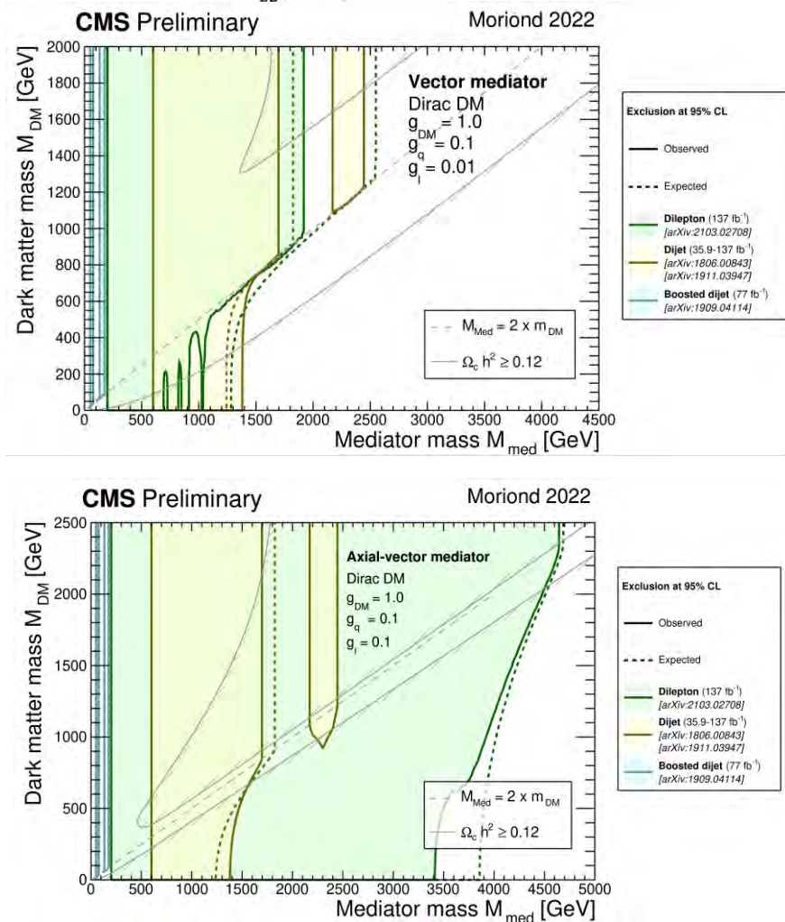
Fig. 15. In the combined channel of the production of a pair of jets and a pair of leptons in the events obtained in the CMS experiment at the LHC, the limits (95% C.L.) were determined on the masses of particle candidates for the role of dark matter particle m_{DM} and the mediator M_{med} . The shaded area corresponds to the excluded mass values for the vector (top) and pseudo-vector (bottom) mediator
