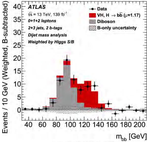
Fig. 14. The invariant mass distribution of a pair of b-jets obtained in pp collisions at an energy of 13 TeV in the ATLAS experiment in the processes of associated production of the Higgs boson with W and Z bosons and its decay into a pair of b-quarks. The contribution from all background processes is subtracted, with the exception of WZ and ZZ
