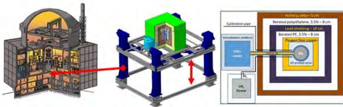
Fig. 18. Scheme of the vGeN setup aimed at detecting CEvNS. The setup is located directly under the KNPP reactor #3 (left), on a special lifting device (center) that allows changing the antineutrino flux in the HPGe detector, surrounded by a complex active and passive shielding (right)
