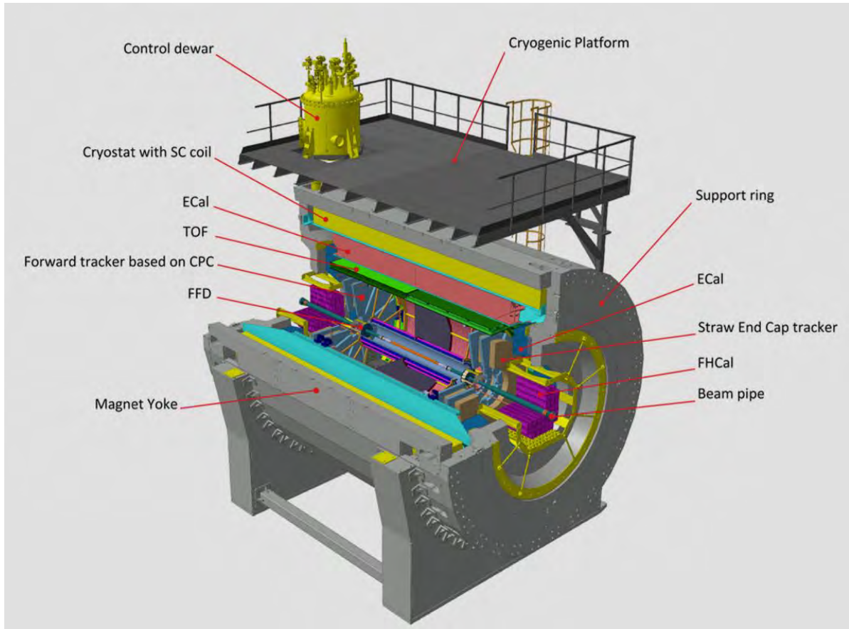
Fig. 4. General scheme of the Multi-Purpose Detector (MPD)
