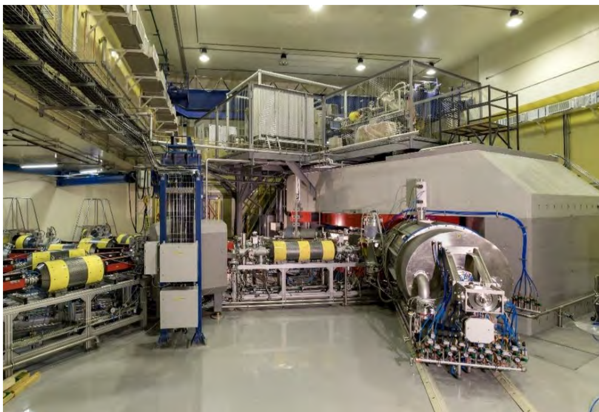
Fig. 19. DC-280 Cyclotron of the SHE Factory
