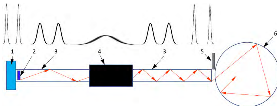
Fig. 24. The idea of an UCN source for a pulsed source using time focusing: 1 – moderator; 2 – UCN converter; 3 – mirror neutron guide; 4 – focusing device; 5 – fast shutter; 6 – UCN trap
