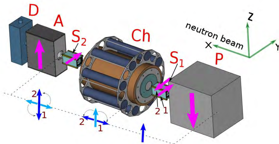
Fig. 22. Scheme of the experiment for measuring T-odd effects in fission. P – SEOP polarizer; Ch – fission chamber surrounded by gamma detectors; A – analyzer; D – neutron detector; S1, S2 – spin control devices. The pink arrows in the figure indicates the direction of the magnetic field, the blue arrows – the direction of the neutron spin
