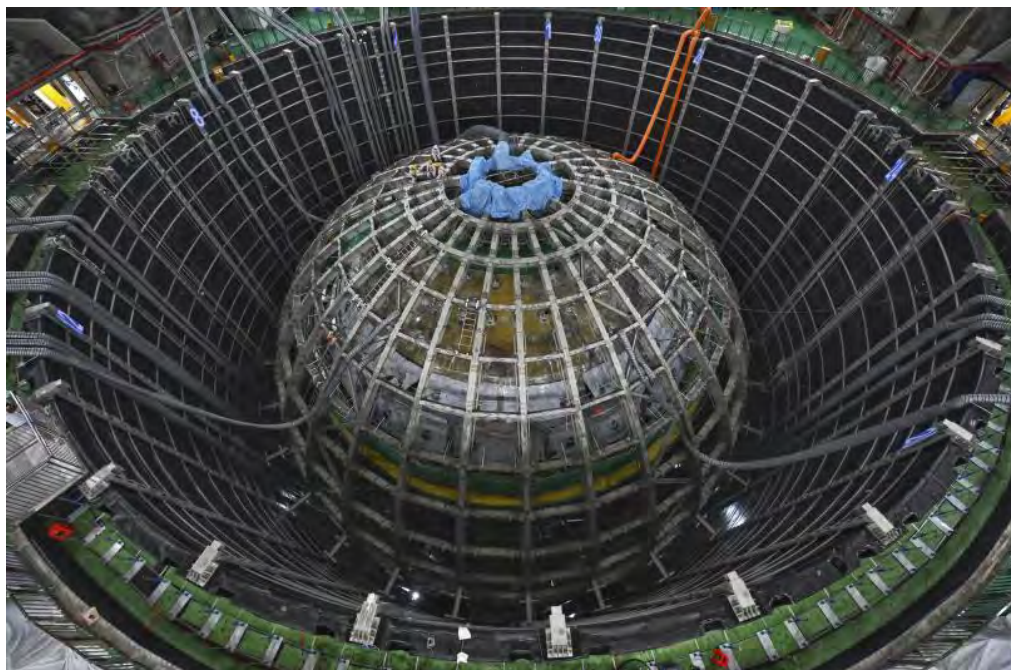
Fig. 16. Current status of the JUNO detector assembly
