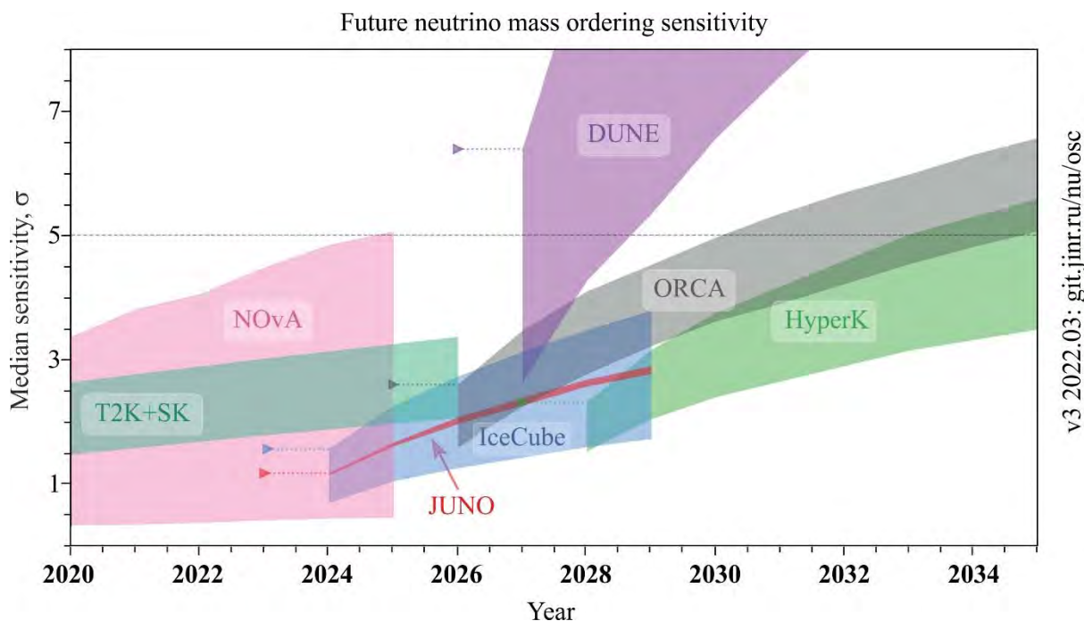
Fig. 17. Neutrino mass ordering sensitivity in current and planned experiments. The bands represent the entire range of possible measurements depending on other parameters
